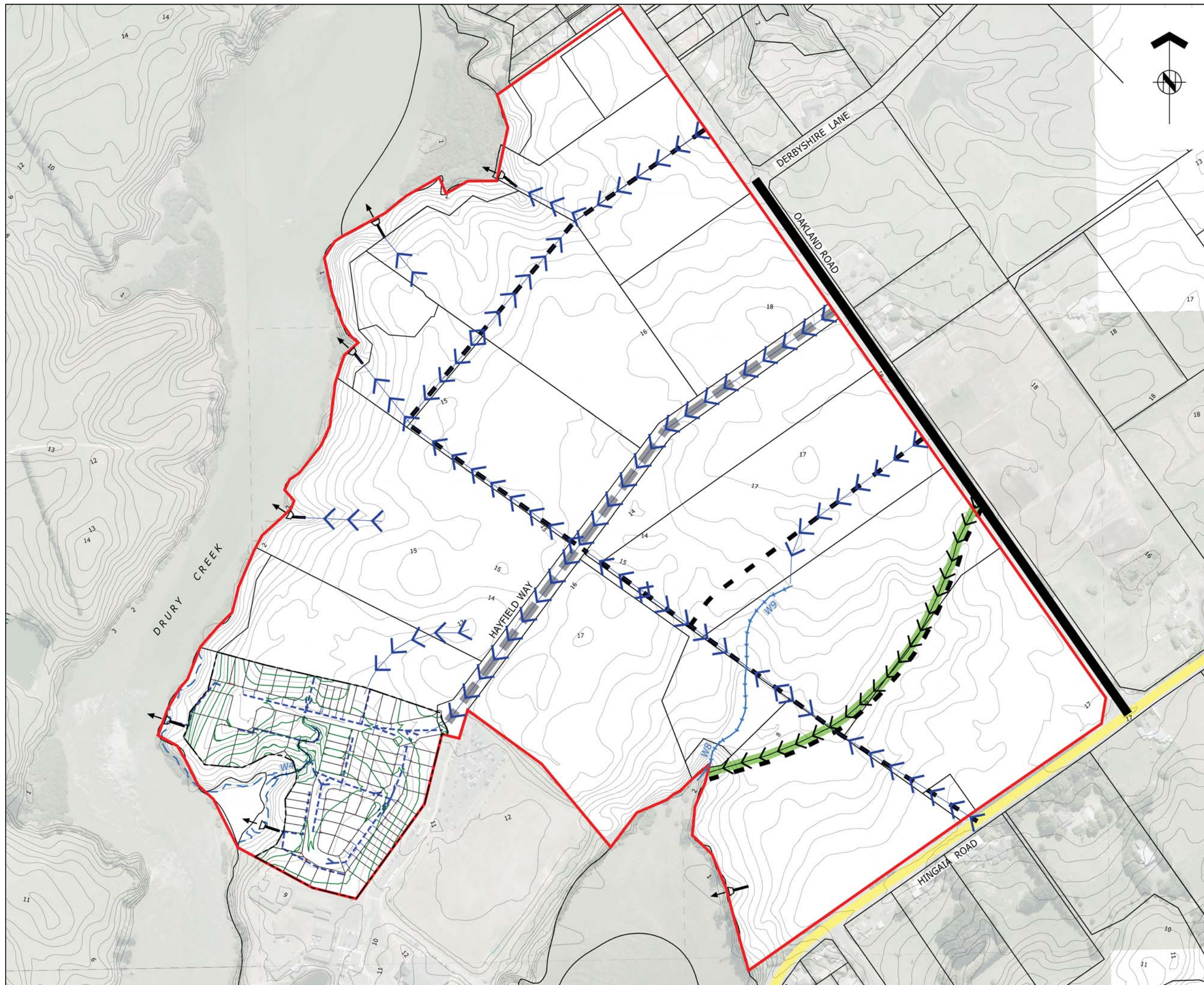
Figure 3b - Stormwater Concept Plan
